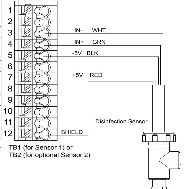
Figure 10 Disinfection Sensor Input Wiring
