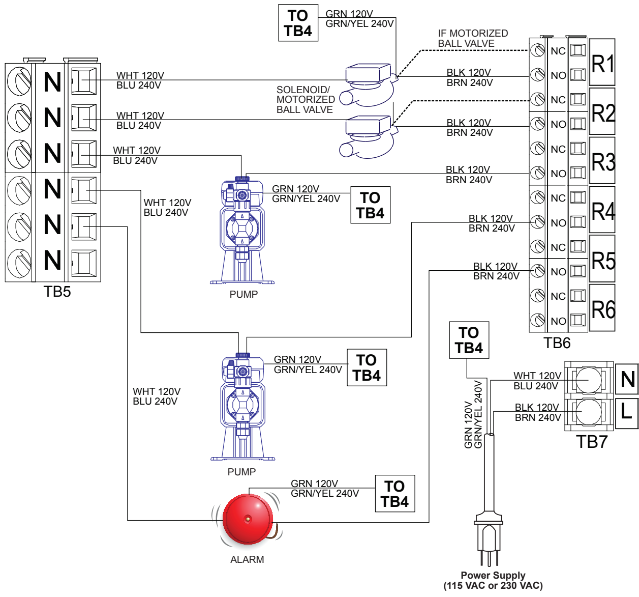
Figure 13 B600 AC Power & Relay Output Wiring
